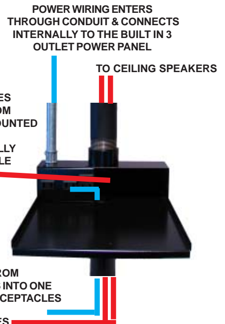
USING CONDUIT FOR THE POWER ENTRY
