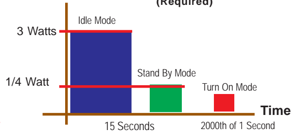
6.3 Amp DC Power Supply (Required)
